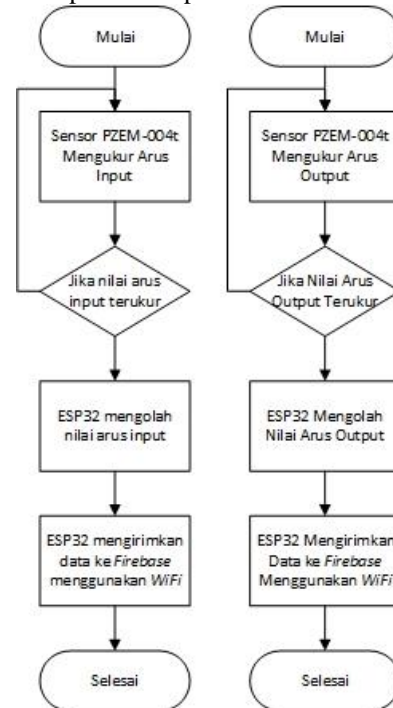
Gambar 2. Flowchart alat
