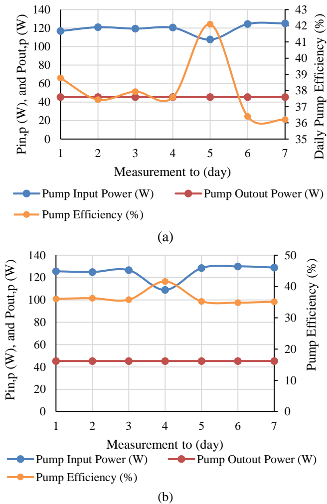
Figure 6. Input power, output power and pump efficiency, (a) morning, and (b) afternoon.
