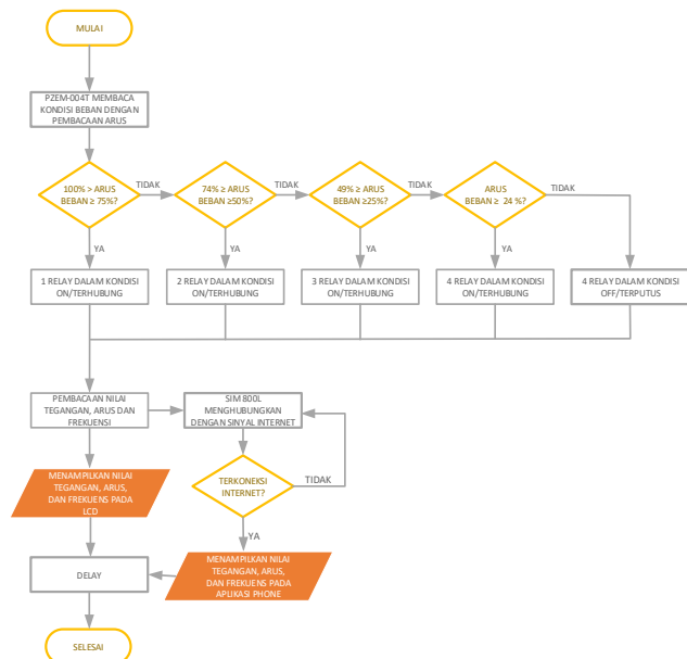
Gambar 3. Flowchart Perancangan Software
