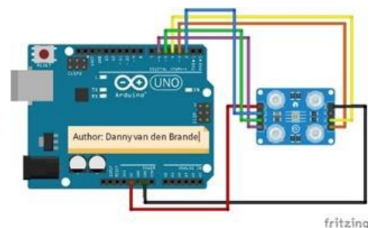
Figure 1. TCS3200 Color Sensor
