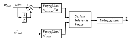
Gambar 9. Model Fuzzy Logic Controller
