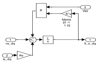
Gambar 5. Model fluks stator motor
