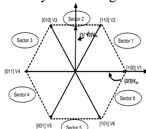
Gambar 2. Mode sektor switching inverter
